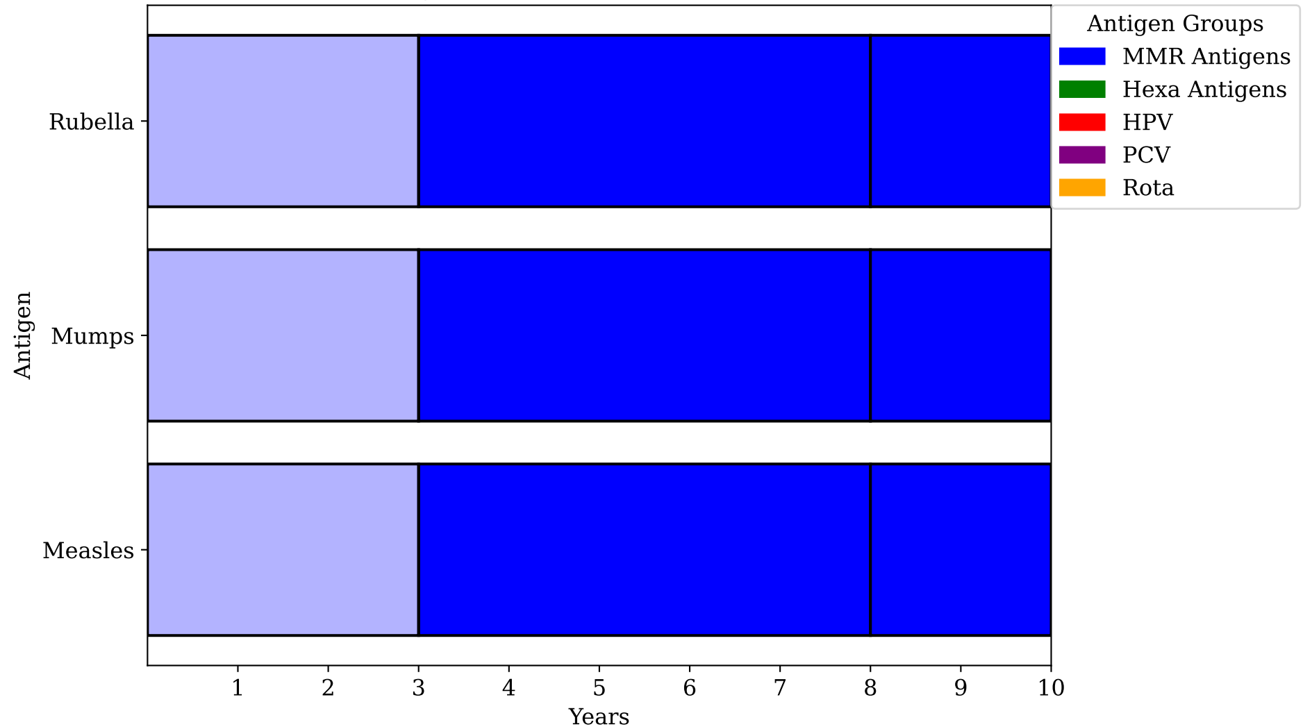
Stochastic Antigen Tender Schedule - Max Profit Phase 1
